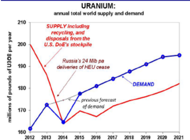
Figure 9 : projected U 3 O 8 supply v. demand
